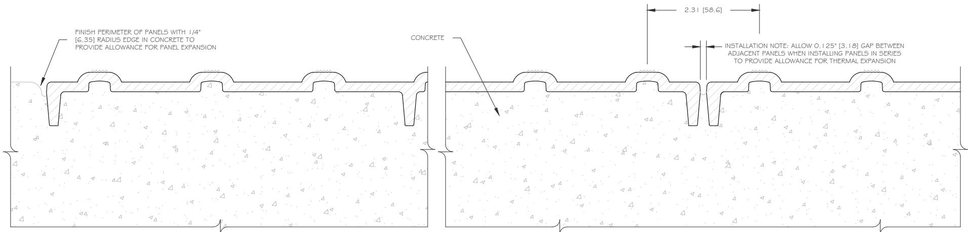
A PERIMETER EMBEDMENT DETAIL
