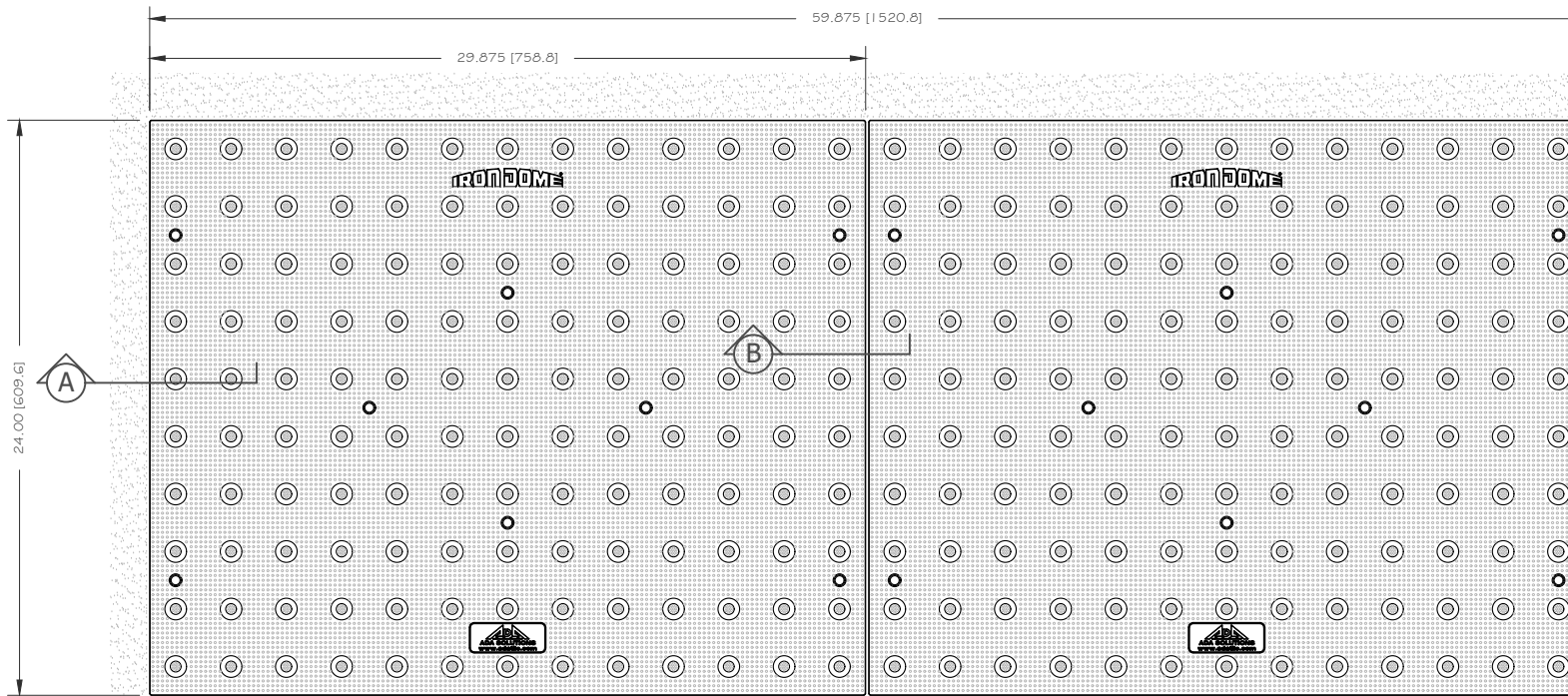
TOP VIEW - MULTIPLE PANEL INSTALLATION (2 PANELS)
