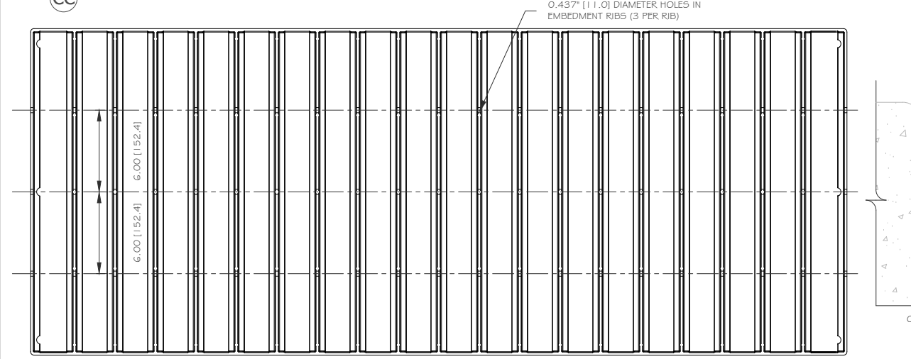
BOTTOM VIEW
