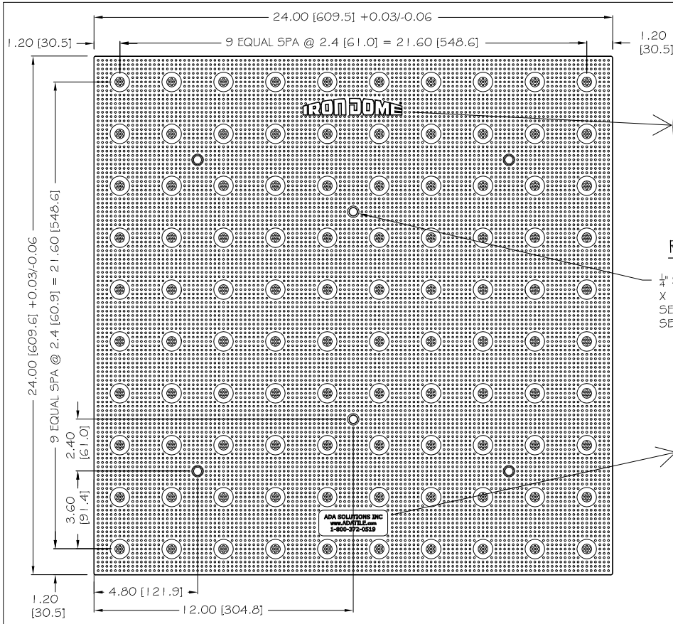
CAST IRON 24X24 TILE TOP VIEW
