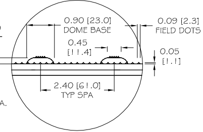
DETAIL 1
