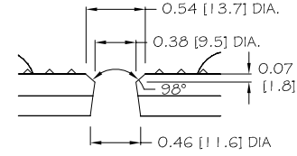
INSERT HOLE DETAIL
