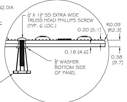
DETAIL 2
