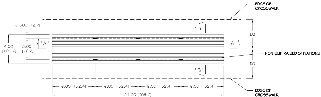
CROSSWALK GUIDE TILE PLAN
