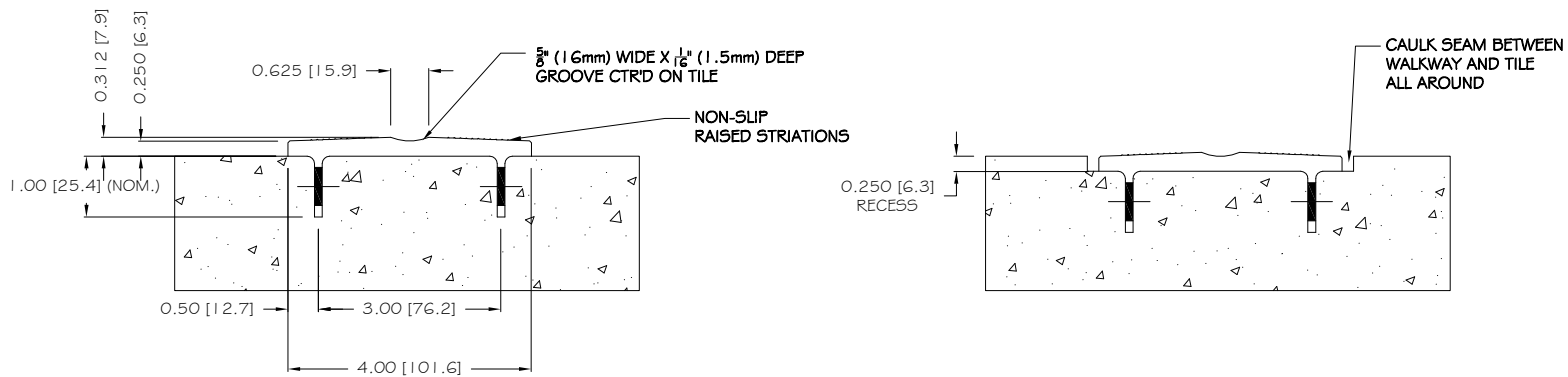
SECTION B-B (NON SNOW REGIONS)
