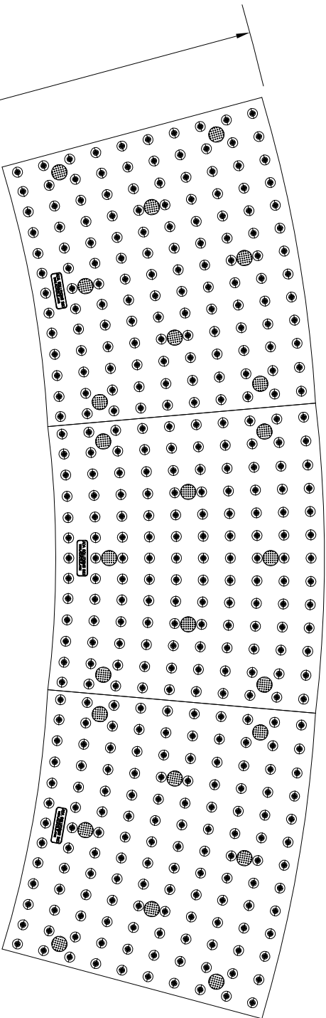
TOP VIEW OF REPLACEABLE PANEL LAYOUT IN A 15' [4.57m] RADIUS
